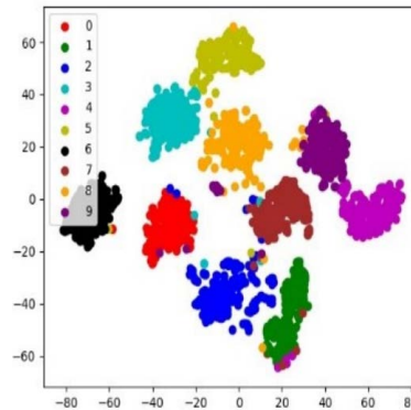
Figure 4: t-SNE visualization of filter weights
